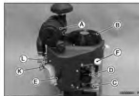
Parts Location
